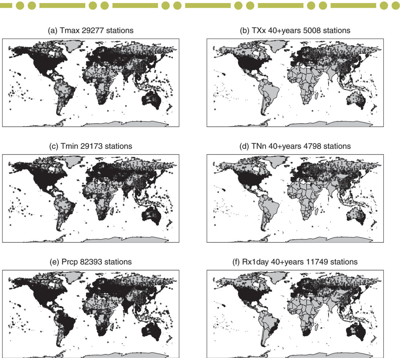
FIG. 1. Locations of station observations in the GHCN-Daily archive. Left-hand side: All stations which provide daily data to calculate the climate indices based on (a) Tmax, (c) Tmin, (e) precipitation. Right-hand side: Stations which provide at least 40 years of calculated index data—for example, (b) TXx based on Tmax, (d) TNn based on Tmin, and (f) Rx1day based on daily precipitation amounts (see Table 1).
