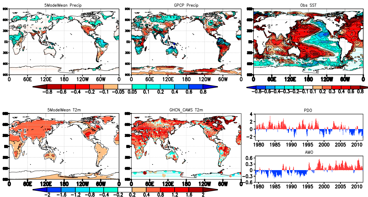
FIG. 3. (top left) Mean simulated precipitation differences ( \text{mm day}^{-1} ) between 1998–2011 and 1979–93, based on results from the five models. (bottom left) Corresponding differences in T2m ( ^{\circ}\text{C} ; land only). (center) As at (left), but for the observations. (top right) The mean observed SST differences ( ^{\circ}\text{C} ) between 1998–2011 and 1979–93. (bottom right) The time series of the PDO ( http://research.jisao.washington.edu/pdo/PDO.latest ) and AMO ( http://www.esrl.noaa.gov/psd/data/timeseries/AMO/ ).
