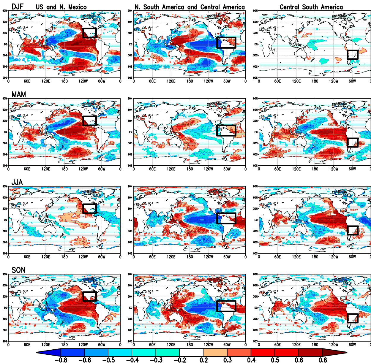
FIG. 5. (left) The correlations between the ensemble mean precipitation averaged over the United States and northern Mexico (black box) and SST for individual seasons (correlations are averaged over the five models). (center) As at (left), but for northern South America and Central America (black box). (right) As at (left), but for central South America (black box).
