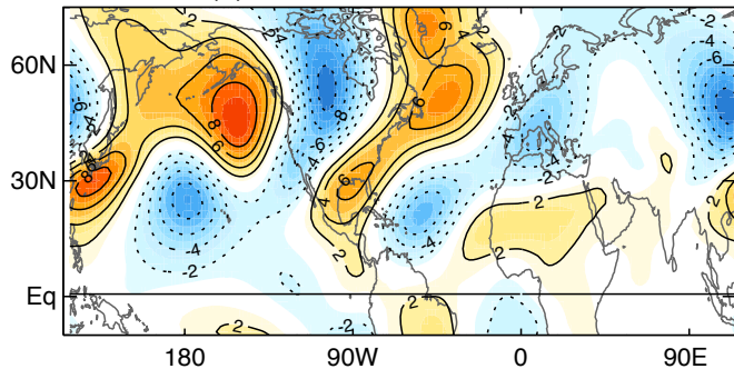
(b) 300hPa v^* , CMIP5, Future-Past
