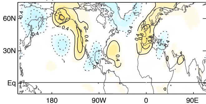
(c) 700hPa v^* , CMIP5, Future-Past
