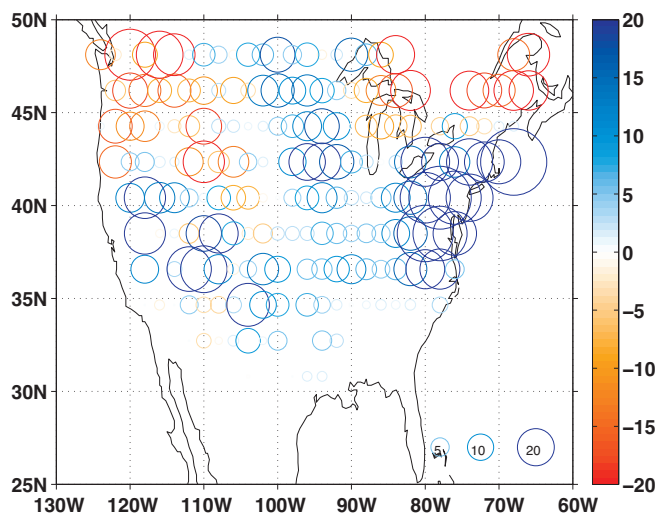
DJF Snowfall (in/season)
