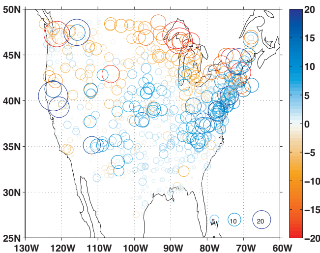
Snowfall (in/season)
