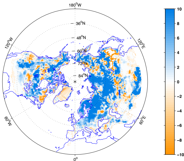
SWE (mm)
