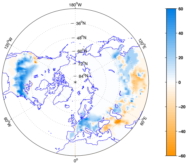
Feb Snow Cover (percent)
