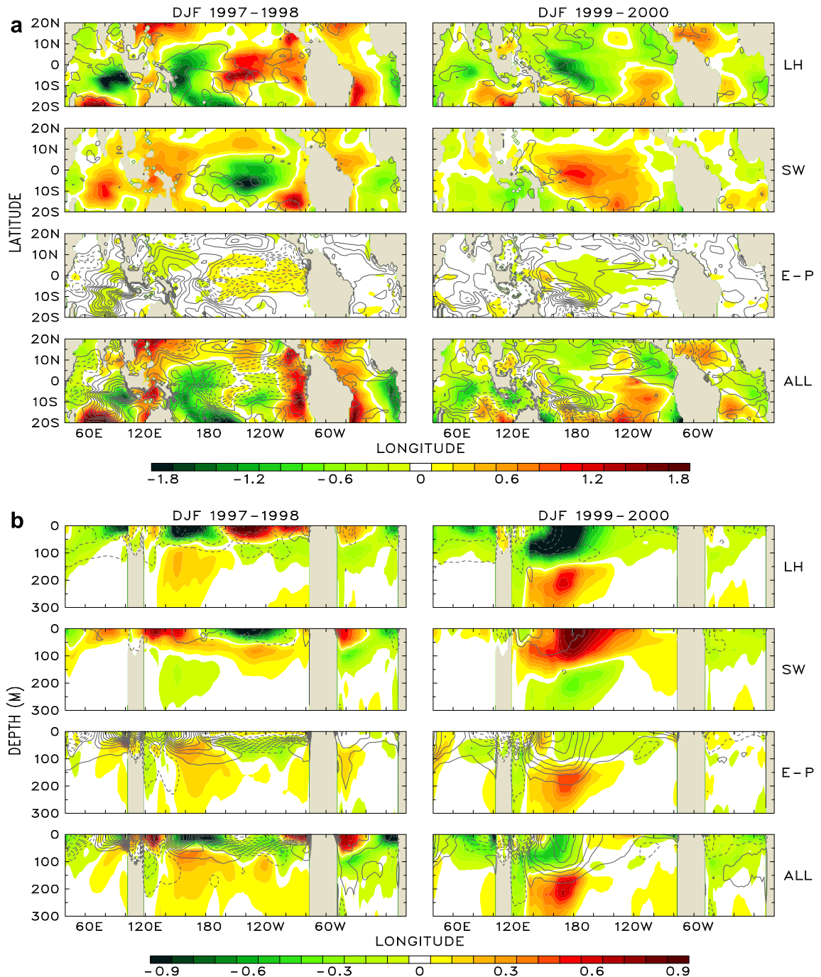
Fig. 7. Impacts of observed anomalous fluxes of latent heat (LH), shortwave radiation (SW) and evaporation minus precipitation (E-P) on tropical temperature and salinity distributions in the Lamont OGCM. Shown in each panel are the differences of temperature (color) and salinity (contours) between model experiments with and without these fluxes. The two columns in (a) display surface maps of winter 1997–1998 and 1999–2000, representing El Nino and La Nina conditions, respectively, while the two columns in (b) are corresponding vertical sections along the equator (5S–5N). The top three rows show the individual effect of each flux whereas the bottom row displays the combined effects of these fluxes. The contour interval for salinity difference is 0.15 for surface plots and is halved for subsurface plots, with solid (dashed) curves for salinity increase (decrease).
