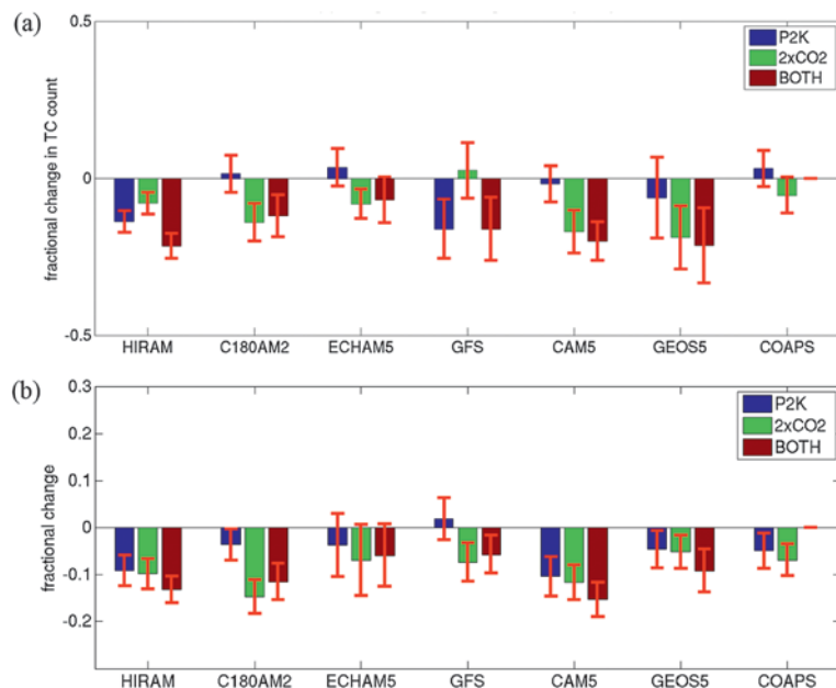
FIG. 3. Comparison between changes in (a) TC formation for various models for the 2K (P2K) and 2xCO 2 experiments vs (b) changes in midtropospheric vertical velocity as weighted by TC genesis, as described in the text. (From Zhao et al. 2013a.)
