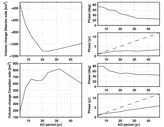
Figure 4. Amplitudes and phases of sea ice volume response to NAM-like forcing anomalies calculated for the Siberian and Canadian sides of the Arctic. Please note that the Siberian side amplitude is shown negative to better indicate its relation to the phase of a positive NAM. The phase of the peak response for both areas changes from mostly in quadrature at short AO periods to more in phase at longer NAM periods.
