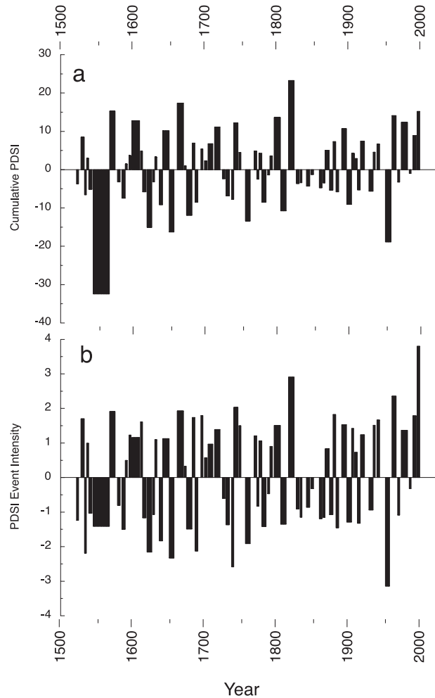
FIG. 4. Temporal distribution of (a) magnitude and (b) intensity of pluvial and drought events 3 years or more in duration. Magnitude portrays the cumulative severity of each event while the intensity indicates the average severity of each event. See text for more details.
