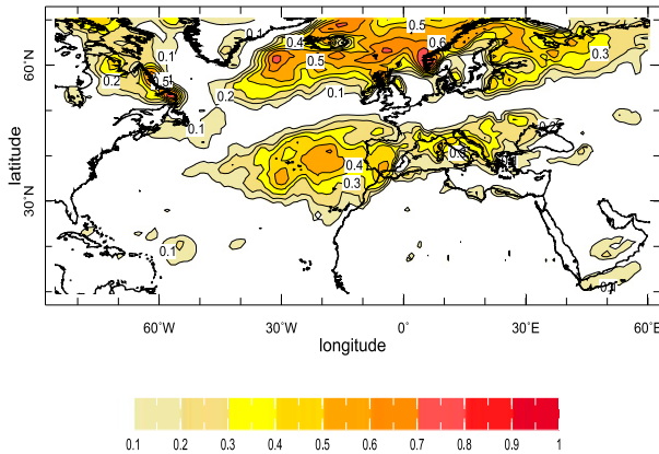
FIG. 2. The fraction of variance in winter (DJFM) precipitation over 1979–2017 explained by the NAO based on ERA-Interim data.
