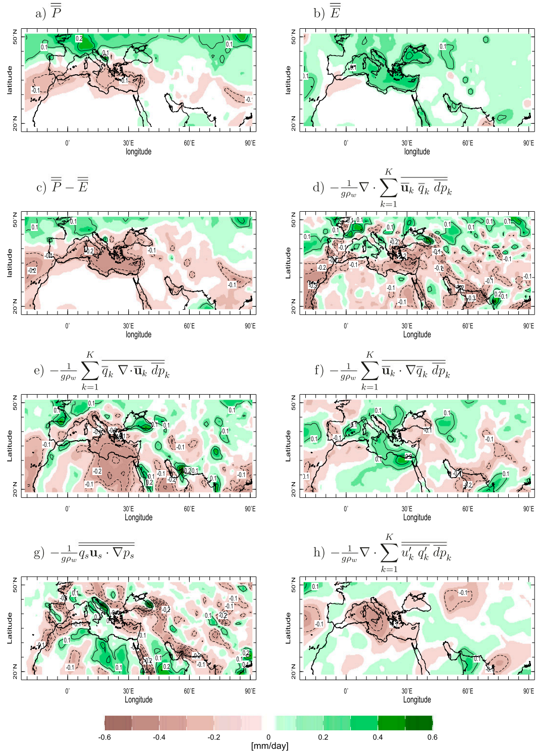
FIG. 11. As in Fig. 10, but for the Mediterranean region.
