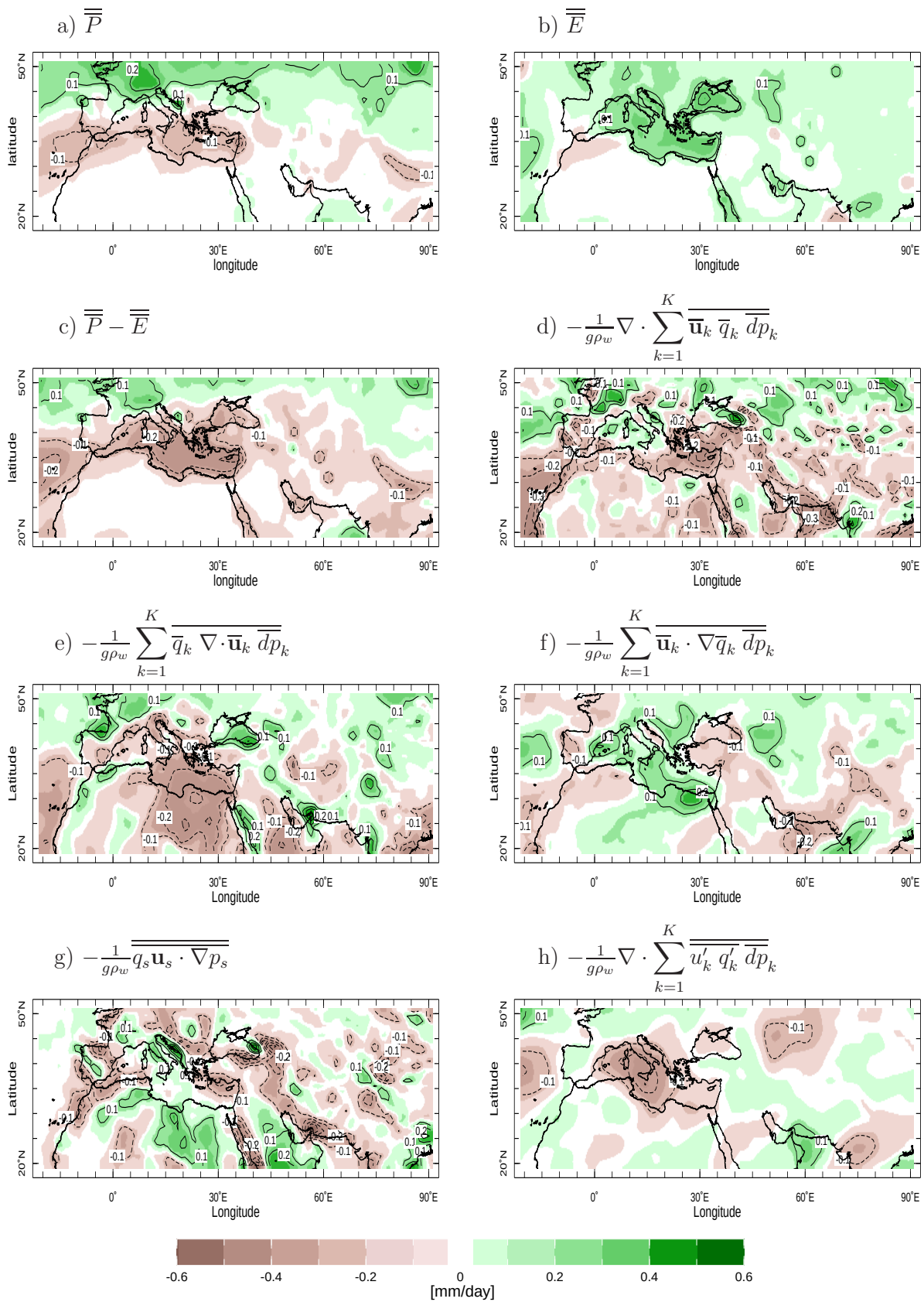
FIG. 11. Same as Figure 10 but for the Mediterranean region.
