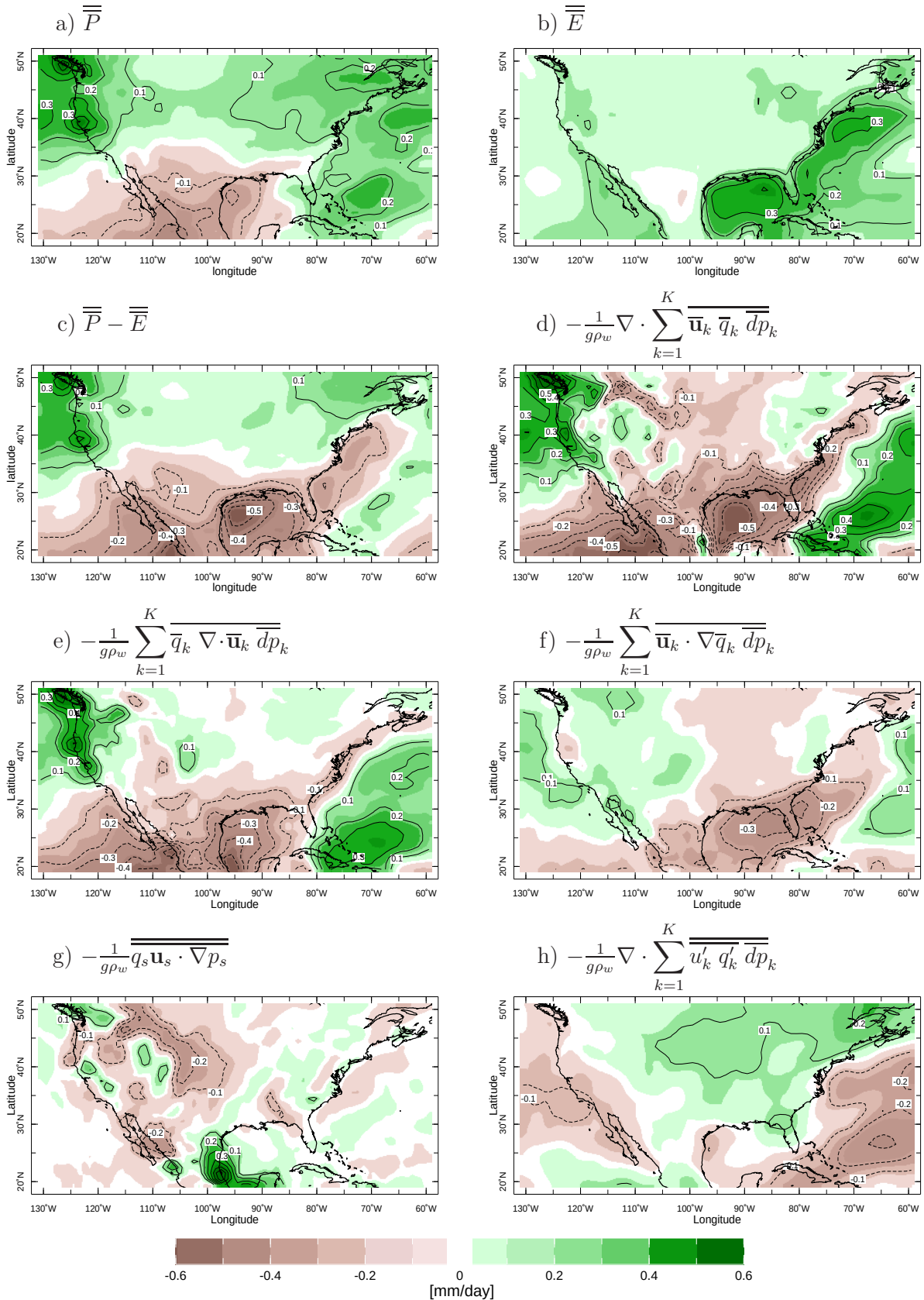
FIG. 10. CMIP5 multimodel mean-projected changes in the winter moisture budget in the North America region for the near term future (2021-2040) minus the recent past (1979-2005) using emissions scenario RCP85 and the historical simulations. Shown are change in a) P , b) E , c) P - E , d) the mean flow moisture convergence, e) the component of d) related to mass divergence, f) the component of d) related to moisture advection, g) the surface term and h) the transient eddy moisture convergence. Units are mm/day.
