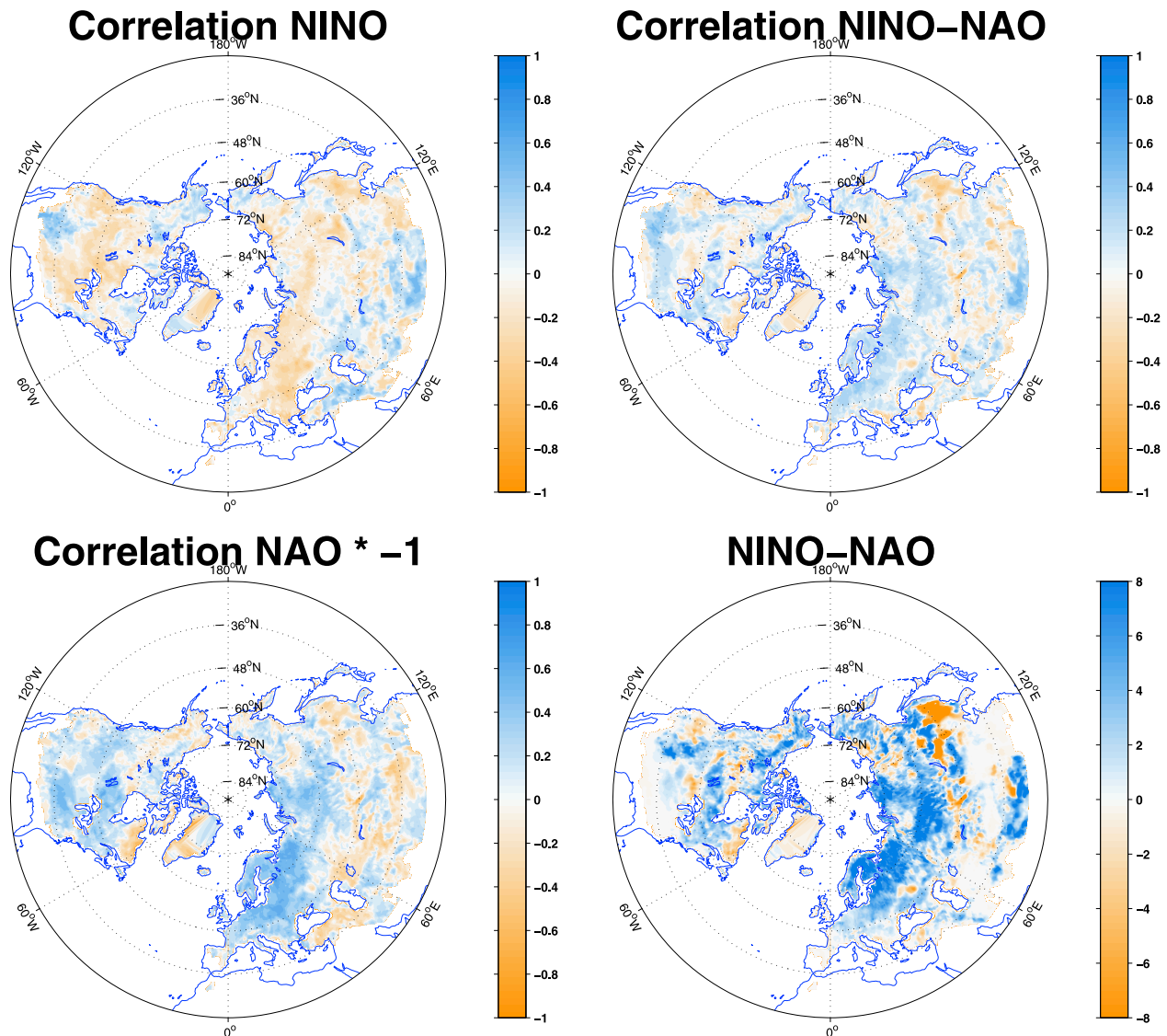
Figure 2. Same as Figure 1 but for snow water equivalent. Units for the regression are mm.
