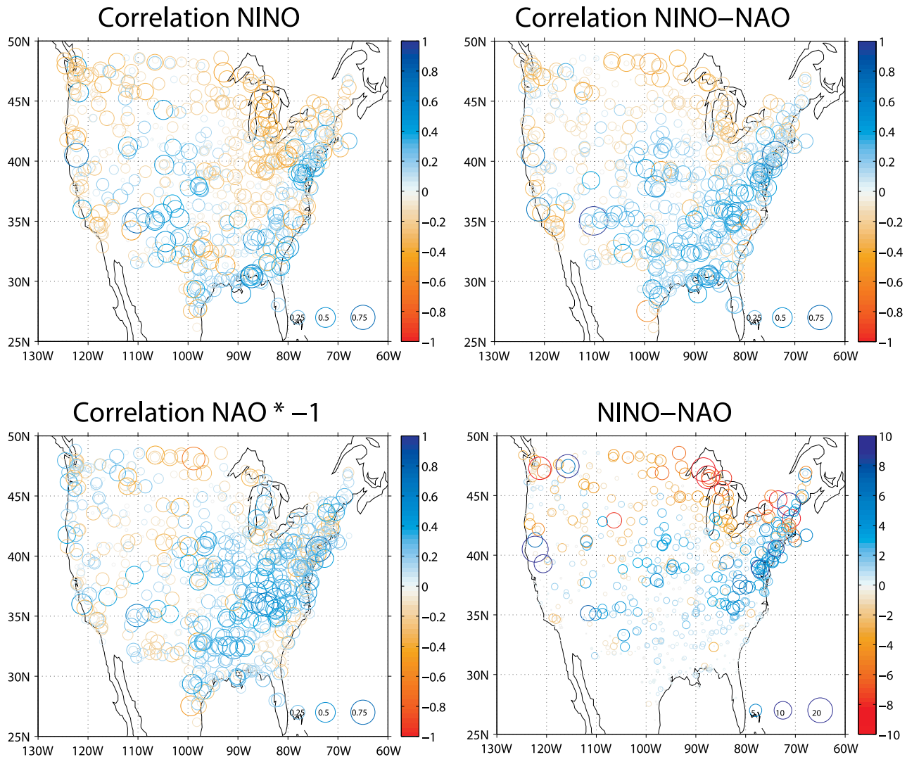
Figure 1. The correlation of snowfall with (top left) the NINO3 index, (bottom left) the NAO index and (top right) the standardized NINO3 minus standardized NAO (NINO-NAO) index and (bottom right) the regression of snowfall on the NINO-NAO index. All indices and the snowfall are for the winter (December to March) mean. Units for the regression are inches.
