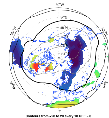
Figure 3. (left) The regression of the 850mb temperature on the NINO3, NAO and NINO-NAO indices (color) with the mean 850mb temperature contoured ( 0^{\circ}\text{C} isotherm bold, negative contours dashed ), and (right) the regression of 300mb submonthly transient eddy meridional velocity variance, v'^2 , all for the December through March seasonal mean. Patterns are plotted only where significant at the 5% level. Units are ^{\circ}\text{C} for temperature and \text{m}^2\text{s}^{-2} for velocity variance.
