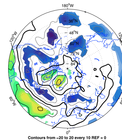
Figure 3. (left) The regression of the 850mb temperature on the NINO3, NAO and NINO-NAO indices (color) with the mean 850mb temperature contoured ( 0^{\circ}\text{C} isotherm bold, negative contours dashed ), and (right) the regression of 300mb submonthly transient eddy meridional velocity variance, v'^2 , all for the December through March seasonal mean. Patterns are plotted only where significant at the 5% level. Units are ^{\circ}\text{C} for temperature and \text{m}^2\text{s}^{-2} for velocity variance.
