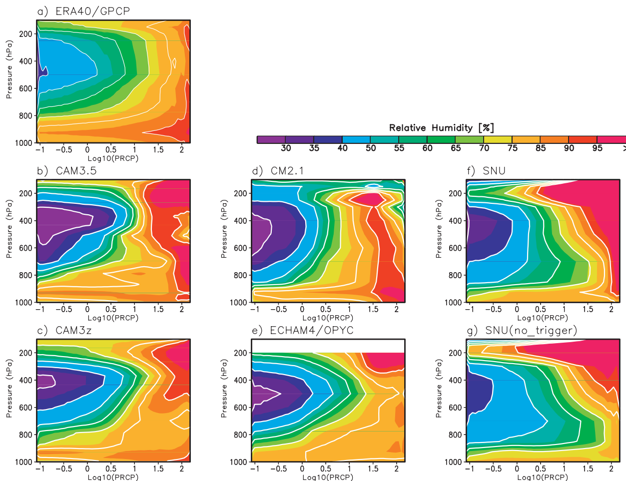
FIG. 13. Composite vertical profile of relative humidity based on precipitation rate: (a) ERA-40/GPCP, (b) CAM3.5, (c) CAM3z, (d) CM2.1, (e) ECHAM4/OPYC, (f) SNU, and (g) SNU without convective inhibition function. The precipitation rate is plotted on a log scale with the relative humidity averaged for each bin shown on the x axis. The data is analyzed over 10^{\circ}\text{S} – 10^{\circ}\text{N} , 40^{\circ} – 220^{\circ}\text{E} .
