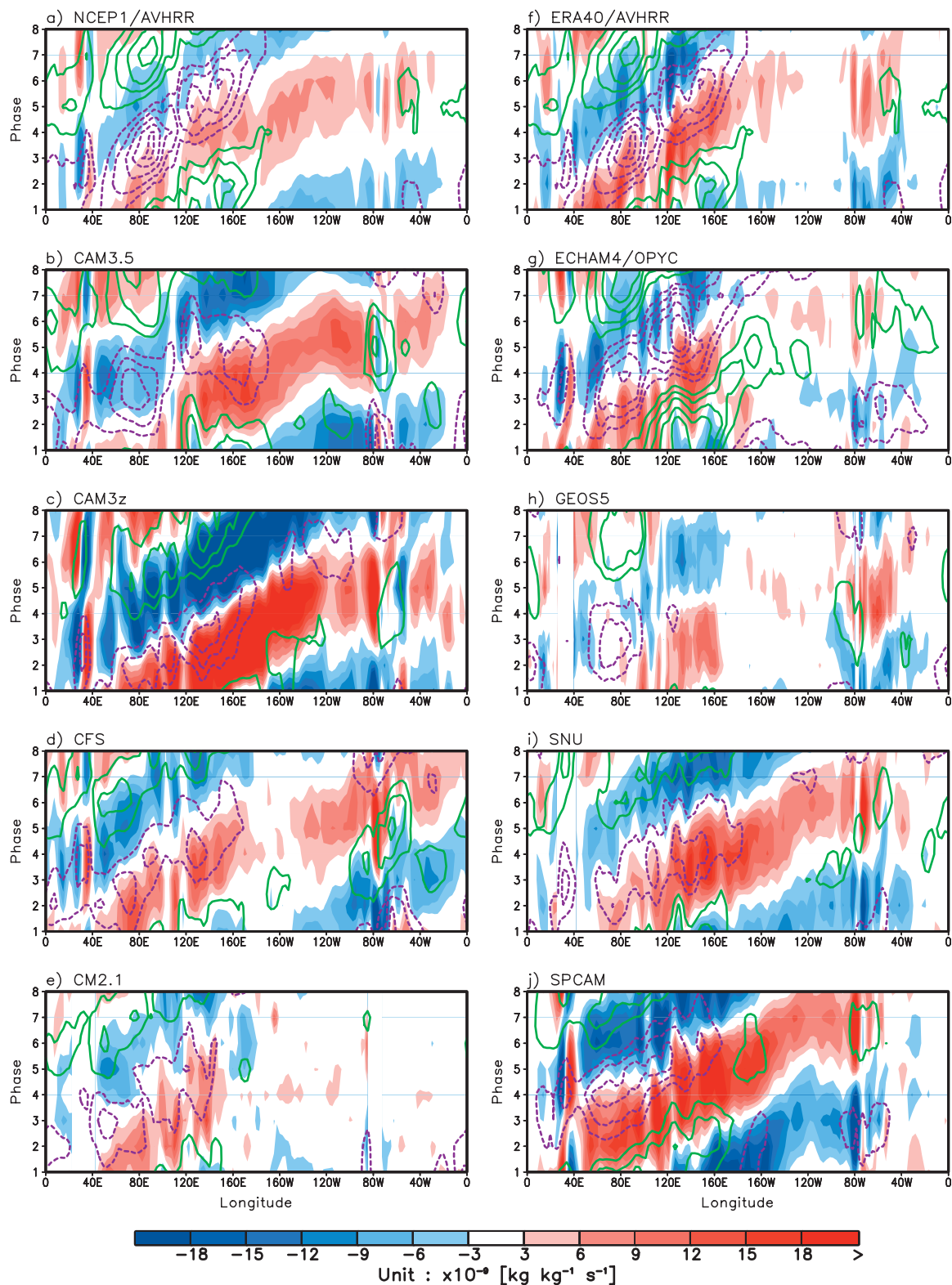
FIG. 10. As in Fig. 9 but for 925-hPa moisture convergence (kg kg -1 s -1 ).
