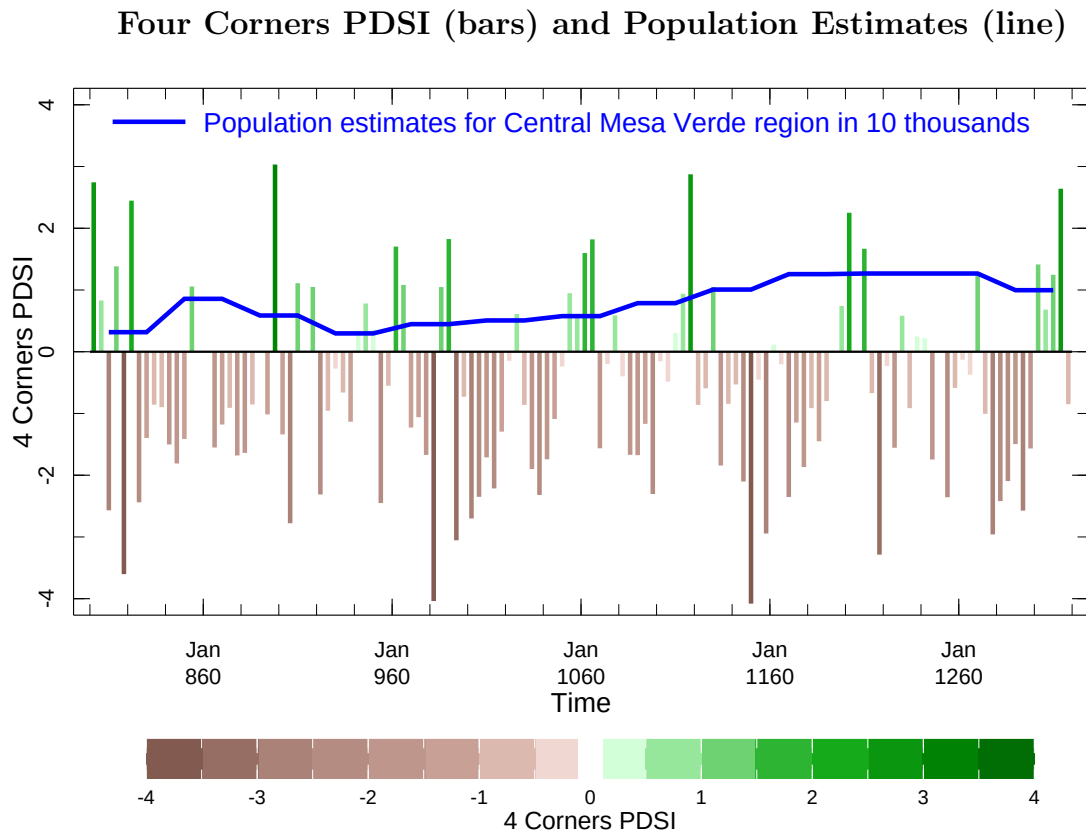
Figure 7: The new tree ring based May-July PDSI reconstructed specifically for the Four Corners region using all available records (and many not in the earlier North American Drought Atlas) covering 800 A.D to 1300 A.D. (bars). The blue line is the population estimate for this region from Wilshusen (2002) plotted in segments of 40 years length.
